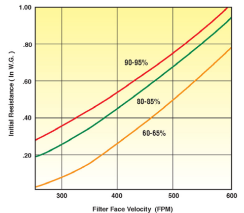
Initial Resistance vs. Filter Face Velocity
