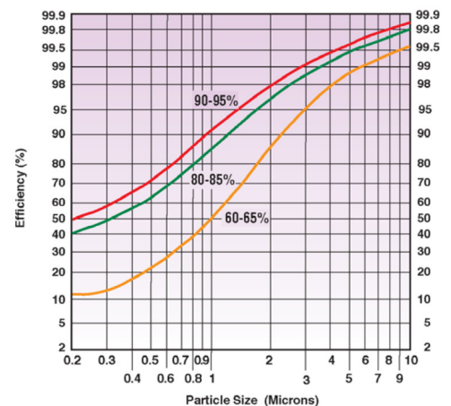
Efficiency by Particle Size
